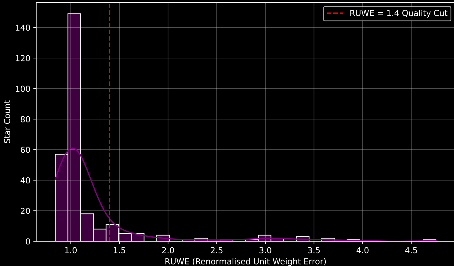
GALAH DR4 Field [6840] RUWE Distribution (n= 275)
